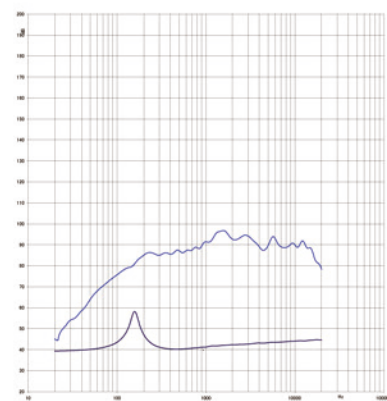
Impedance Curve
